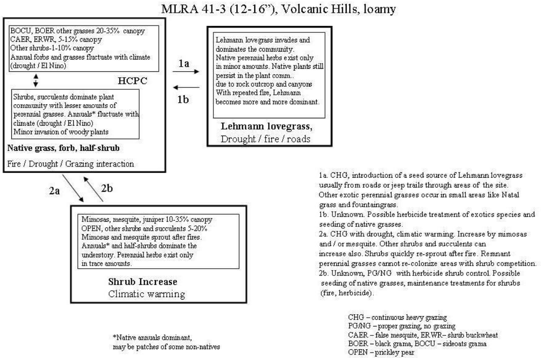
Figure 12. State and transition model for Volcanic Hills, loamy
